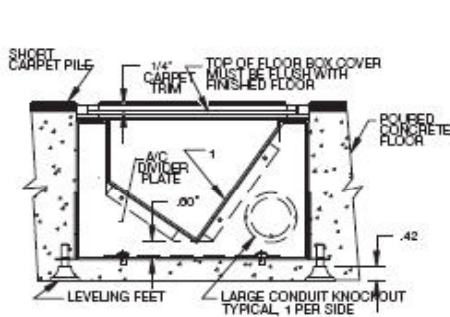
Installation Cross Section
